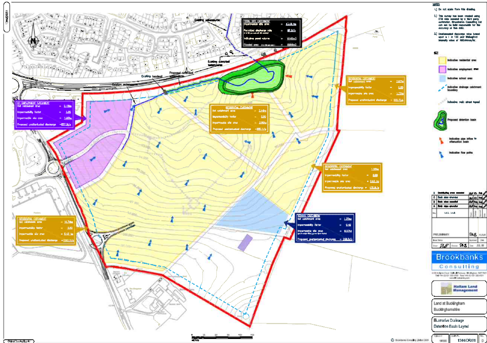
Figure 4.4 Proposed surface water attenuation basin in the north of the Lace Hill Development
